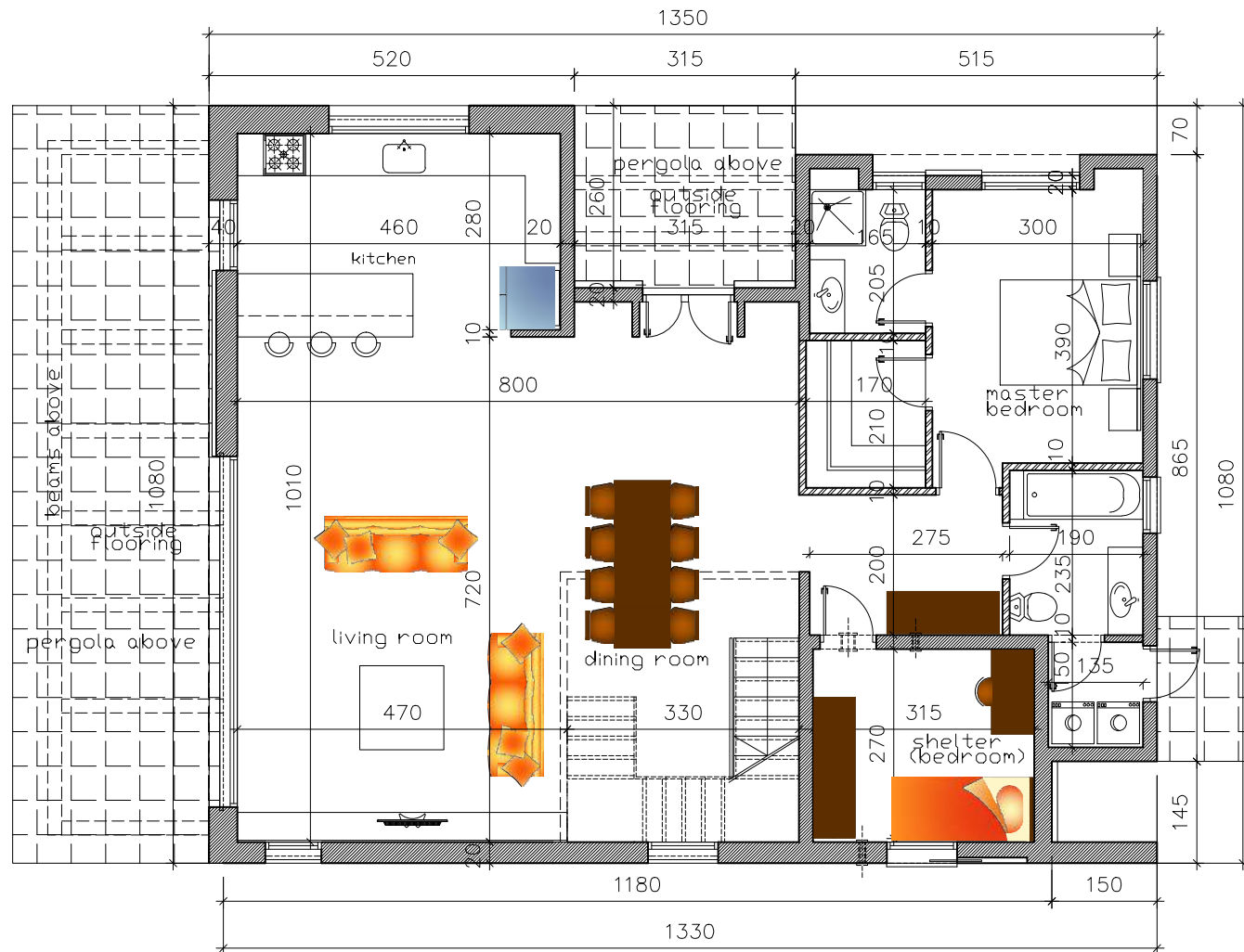
1 st floor 131 m 2 scale 1:100
